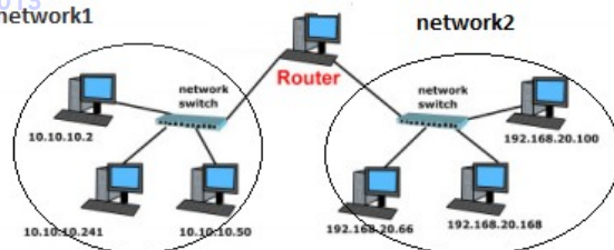
Fig 11.5 Router
